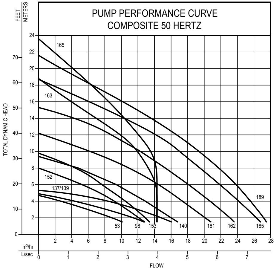
TOTAL DYNAMIC HEAD/FLOW EFFLUENT AND DEWATERING
